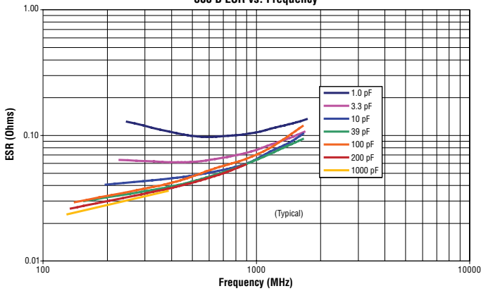
800 B ESR vs. Frequency
