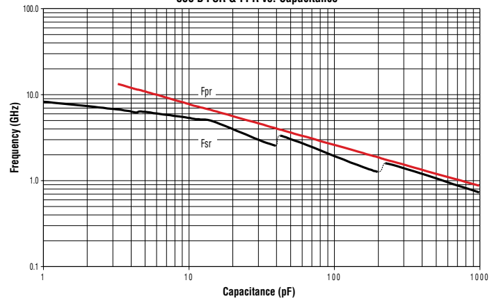
800 B FSR & FPR vs. Capacitance
