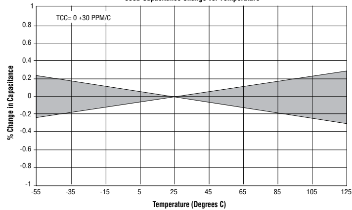
800B Capacitance Change vs. Temperature
